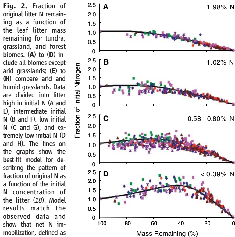
Fig. 2. Fraction of original litter N remaining as a function of the leaf litter mass remaining for tundra, grassland, and forest biomes. (A) to (D) include all biomes except arid grasslands; (E) to (H) compare arid and humid grasslands. Data are divided into litter high in initial N (A and E), intermediate initial N (B and F), low initial N (C and G), and extremely low initial N (D and H). The lines on the graphs show the best-fit model for describing the pattern of fraction of original N as a function of the initial N concentration of the litter (18). Model results match the observed data and show that net N immobilization, defined as an absolute increase in N concentration of the litter, is highest for the leaf litter with very low initial N concentration and decreases to minimal values for high initial N concentration of leaf litter. Leaf litter in arid grasslands was an exception showing no N immobilization in the low and very low N litters.
